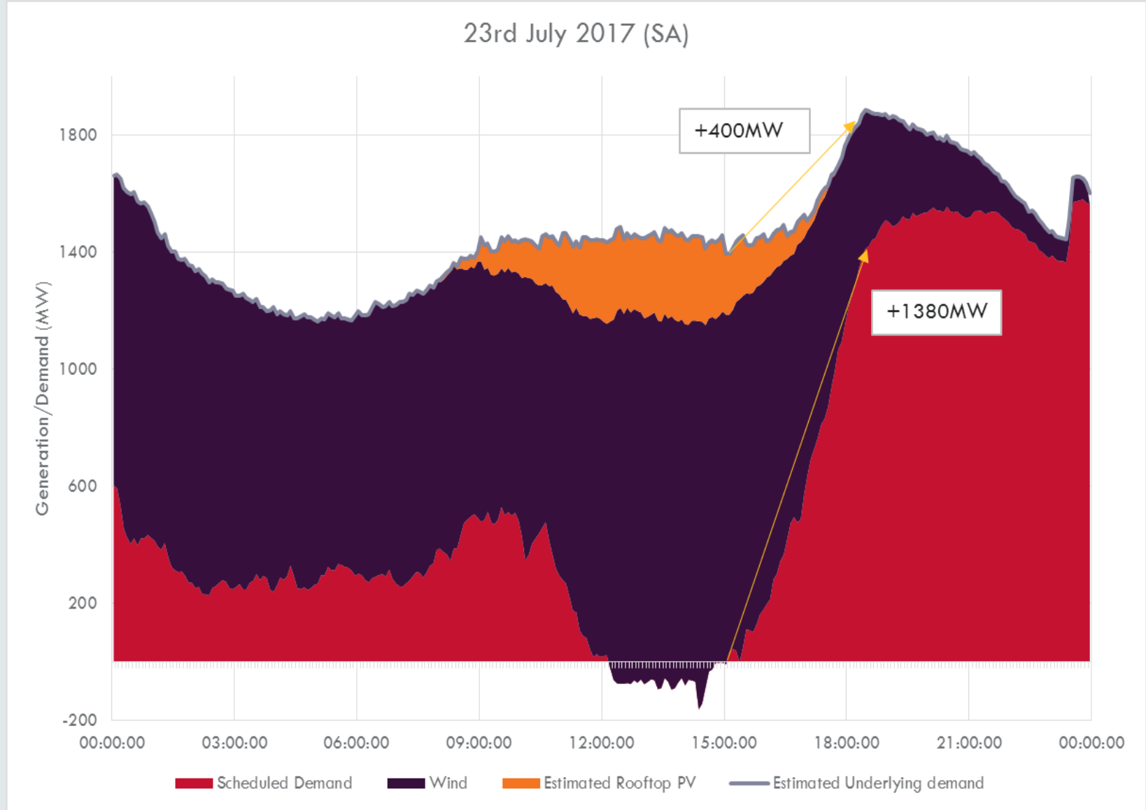
Flexible plant ramping, South Australia, Sunday 23 July 2017
